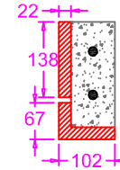
Structural Reinforced Concrete Backing
