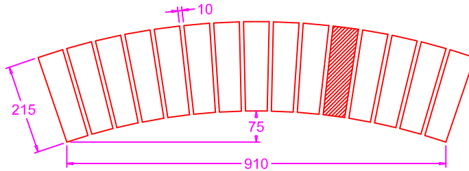
Single Piece Segmental Arch
