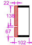
Non-Structural Polystyrene Backing
