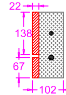
Non-Structural Lightweight Concrete
