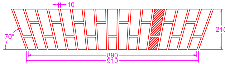
Flat Gauged Skew Based Arch
