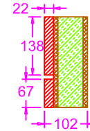
Non-Structural cement particle board with Polytherane core
